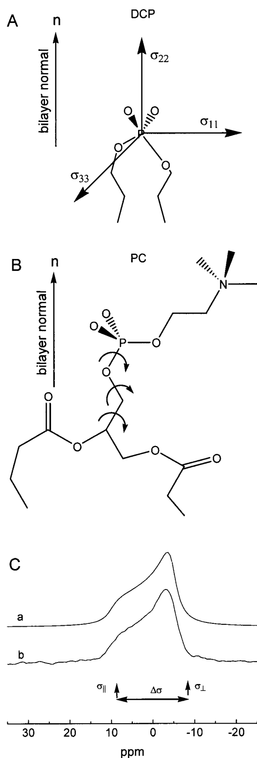
FIGURE 7 Different orientation of the diester phosphate group of DCP ( A ) and phosphatidylcholine ( B ) in a bilayer with respect to the bilayer normal, n . The orientation of the shielding tensor is shown for DCP ( A ). Arrows indicate possible intramolecular rotations of the phosphatidylcholine headgroup, which can reduce the CSA ( B ). Simulated ( a ) and experimental ( b ) ^{31}\text{P} NMR spectra are shown for DCP in the L_\alpha lamellar phase ( C ). The simulated spectrum was obtained by using \Delta\sigma = 15 ppm and 200-Hz line broadening.
