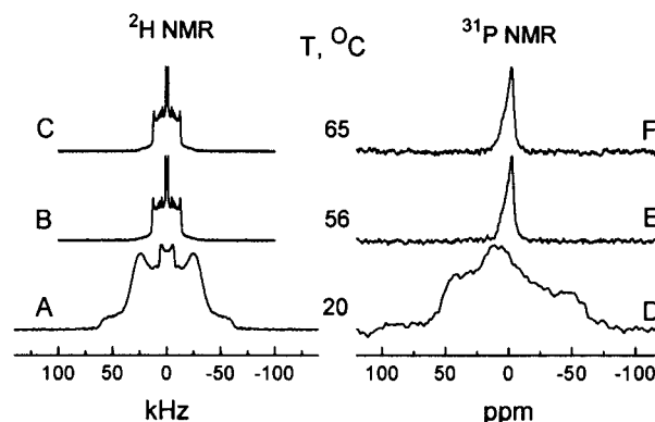
FIGURE 5 ^2\text{H} NMR (A–C) and ^{31}\text{P} NMR (D–F) spectra of [^2\text{H}_{35}] -MSG:DCP, 9:1 (mol/mol) in the presence of \beta -lactoglobulin at different temperatures. Lipid:protein ratio, 100:1 (mol/mol); pH 7; 0 mM NaCl.
