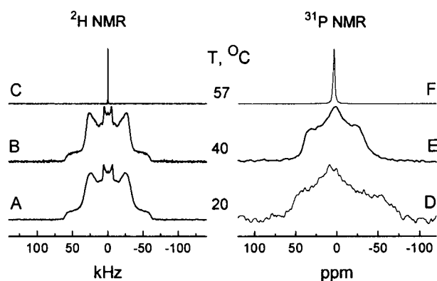
FIGURE 4 ^2\text{H} NMR (A–C) and ^{31}\text{P} NMR (D–F) spectra of [^2\text{H}_{35}] -MSG:DCP, 9:1 (mol/mol) at different temperatures, as indicated in the figure.
